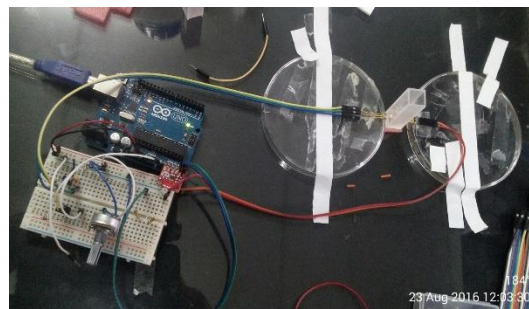
Figure 1. The circuit sensor blood glucose meter.
