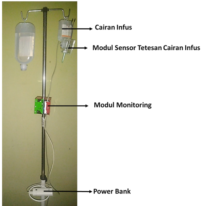
Figure 7. Infusion Fluid Monitoring System
