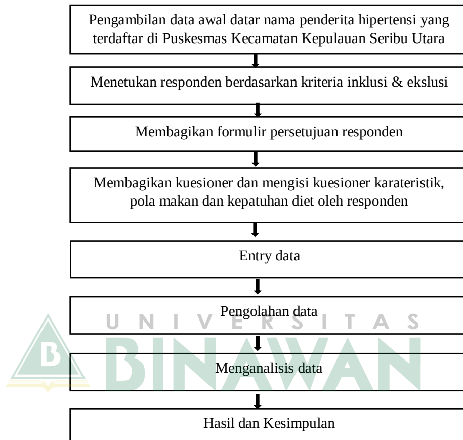
Gambar 3. Alur Penelitian
